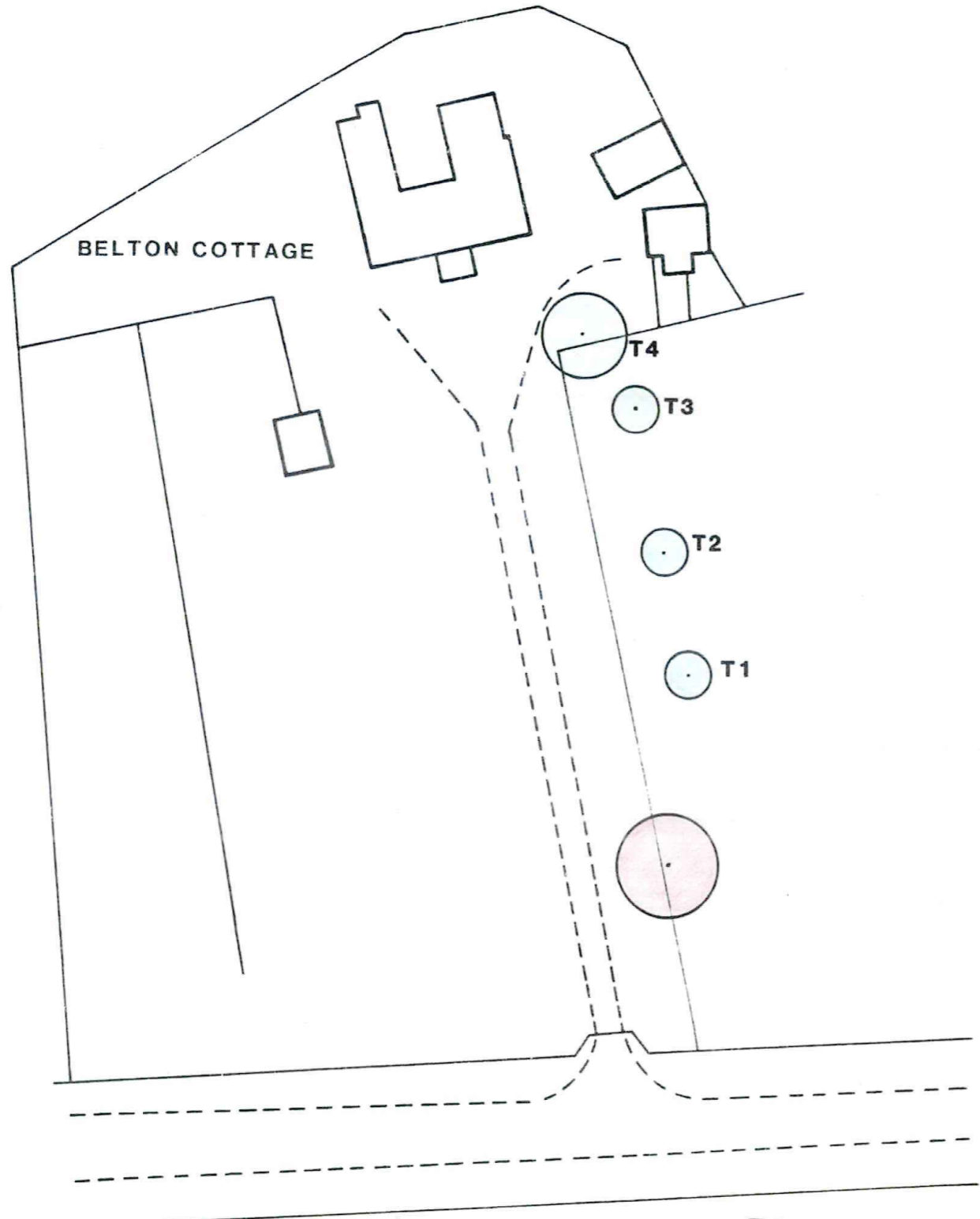
Block Plan 1/500
